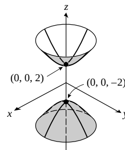
21. Hyperboloid of two sheets
